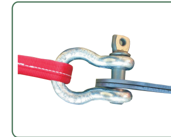
BOW Shackle
